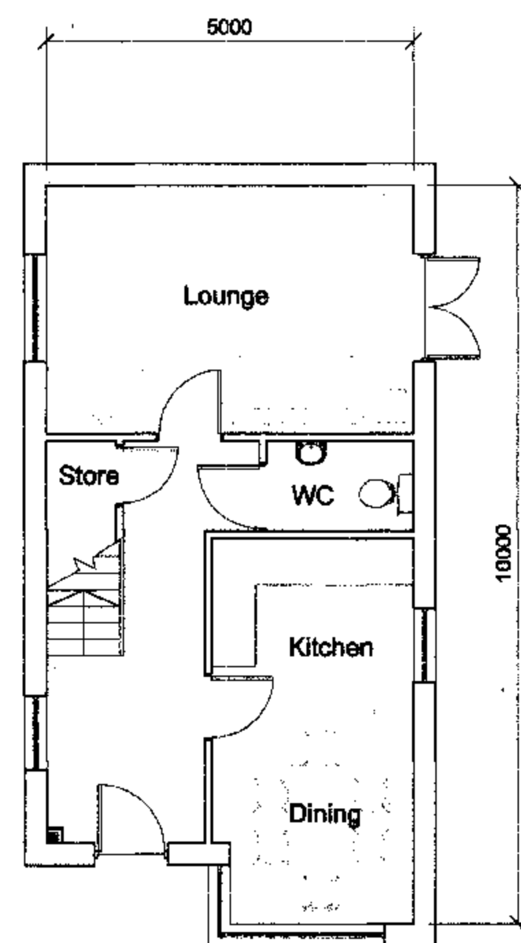
GROUND FLOOR
